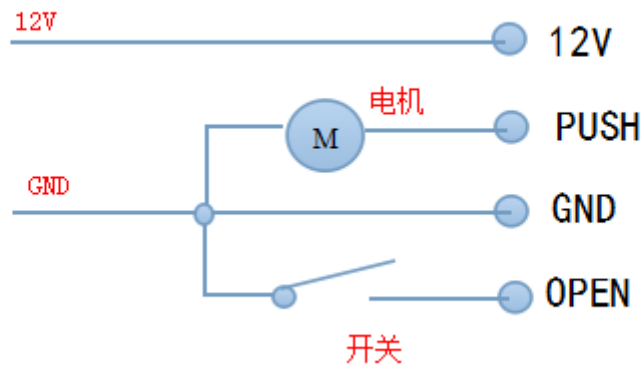
Connection Diagram
